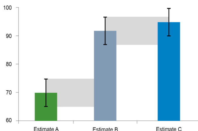
Figure 2 Confidence intervals
